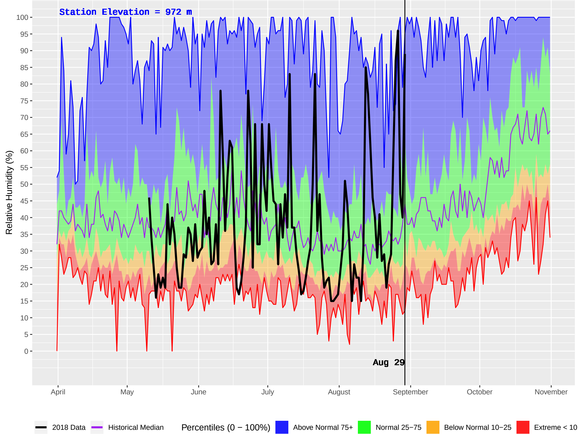
SPARKS LAKE (305) : Historical (1991–2016) and Current (2018) Daily Relative Humidity
