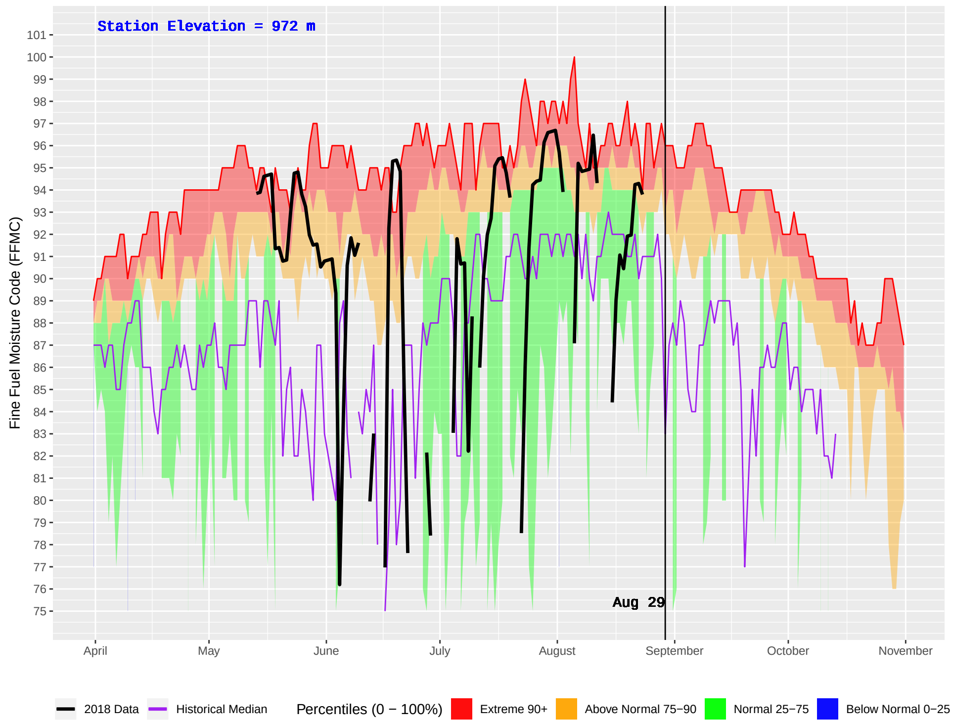
SPARKS LAKE (305) : Historical (1991–2016) and Current (2018) Daily Fine Fuel Moisture Code (FFMC)
