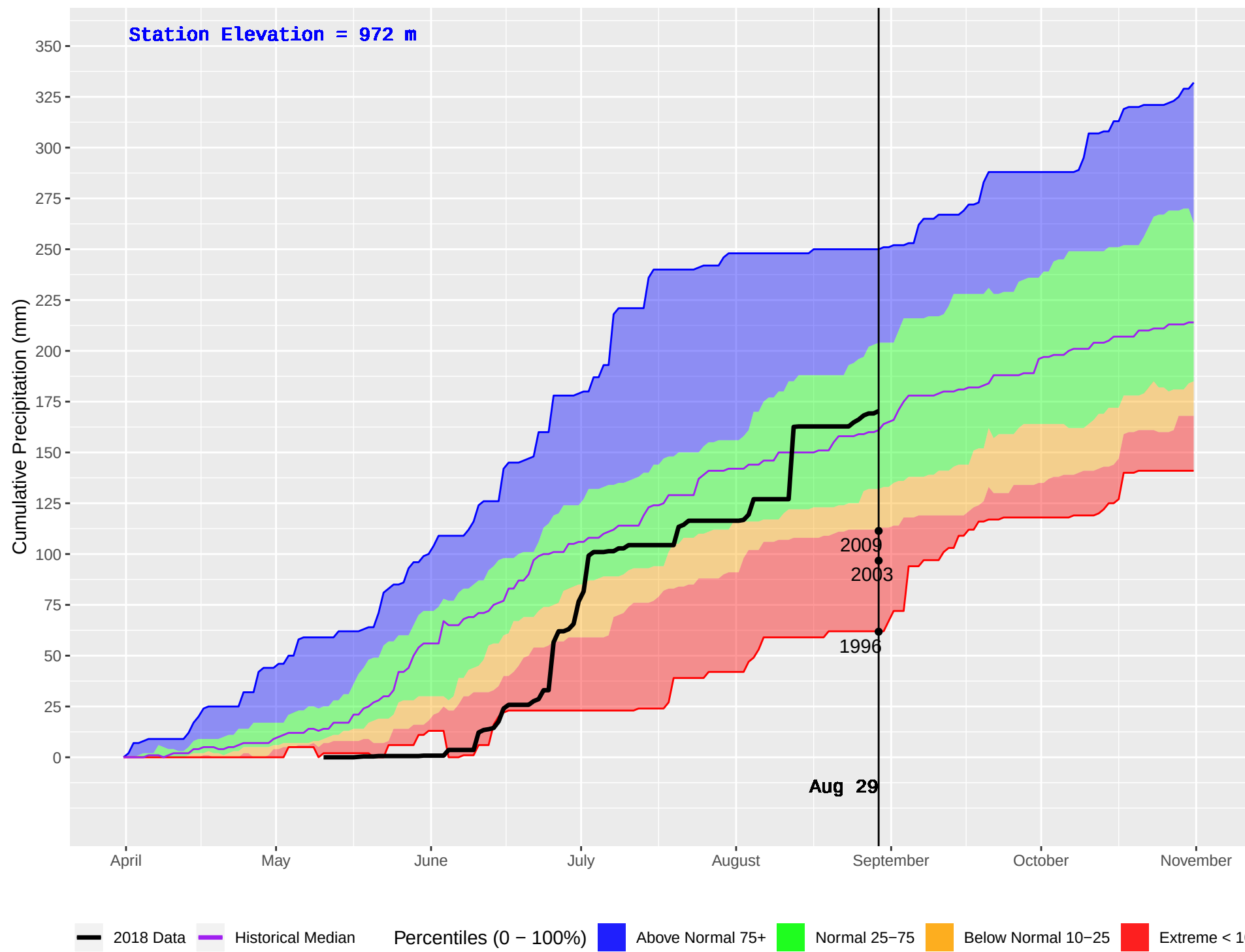
SPARKS LAKE (305) : Historical (1991–2016) and Current (2018) Daily Cumulative Precipitation
